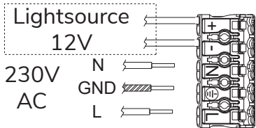
Internal connection
